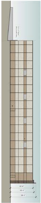
4 EAST ELEVATION
